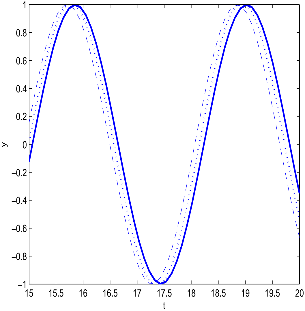
Exact Solution with y_0 and y_0 + \varepsilon y_1
