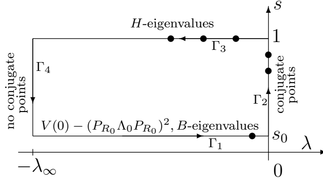
FIGURE 1. Schematic of the path \Gamma = \Gamma_1 \cup \Gamma_2 \cup \Gamma_3 \cup \Gamma_4
