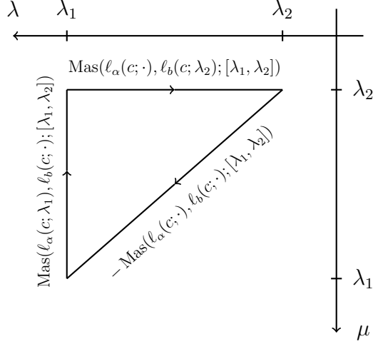
Figure 4.2: Triangular path in the (\lambda, \mu) -plane for Claim 4.1.
