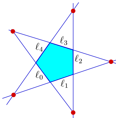
Fig. 4. The base points of \beta
