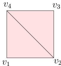
Fig. 5. A triangulation of a quadrilateral
