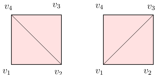
Fig. 6. Triangulations of Quadrilateral
