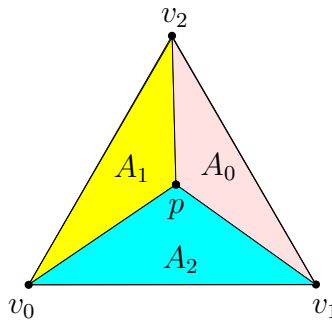
Fig. 1. Barycentric coordinates for a triangle
