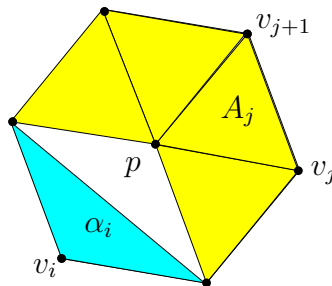
Fig. 3. Wachspress coordinates for a polygon
