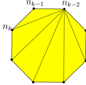
Fig. 8. Triangulation used for adjoint
